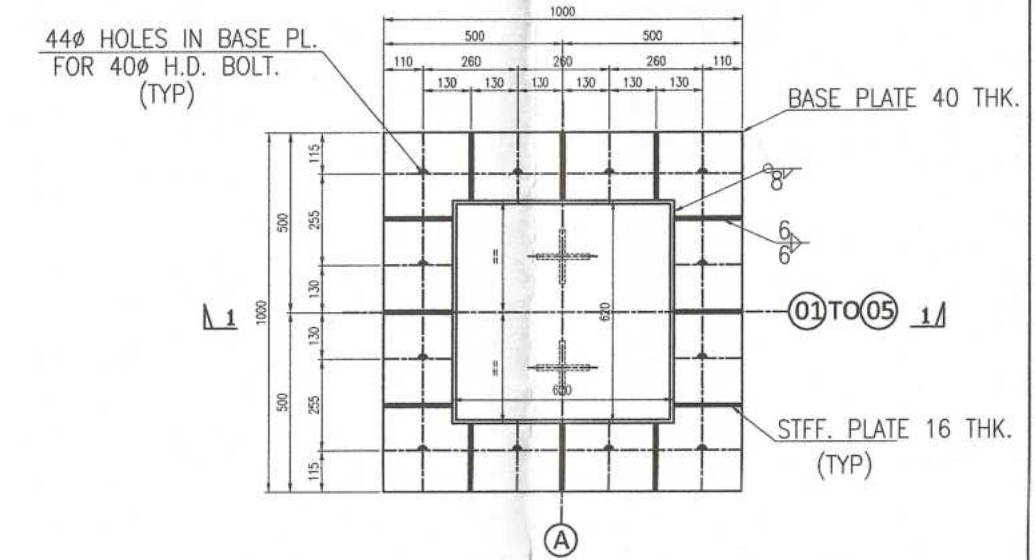
BASE DETAIL FOR COLUMN MKD. C1
