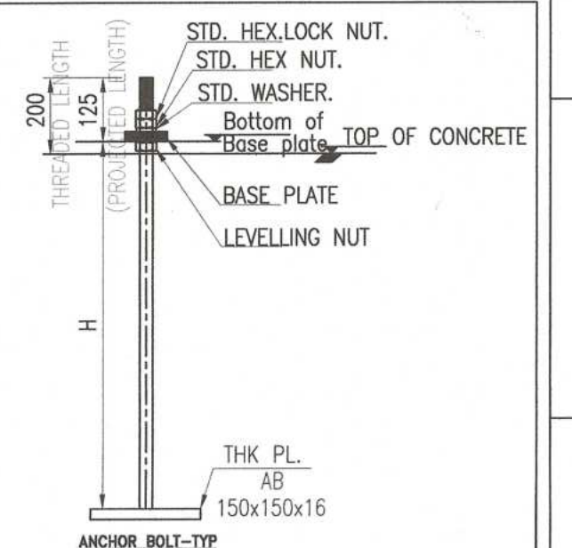
WITH LEVELLING NUT
