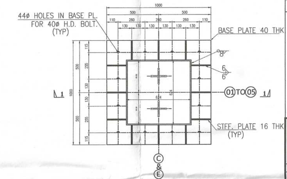
BASE DETAIL FOR COLUMN MKD. C3
