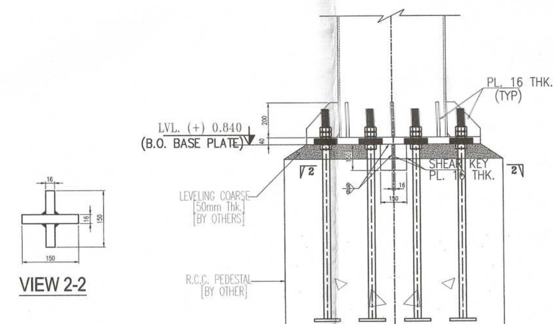
BASE DETAIL FOR COLUMN MKD. C4
