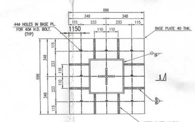
BASE DETAIL FOR COLUMN MKD. C4
