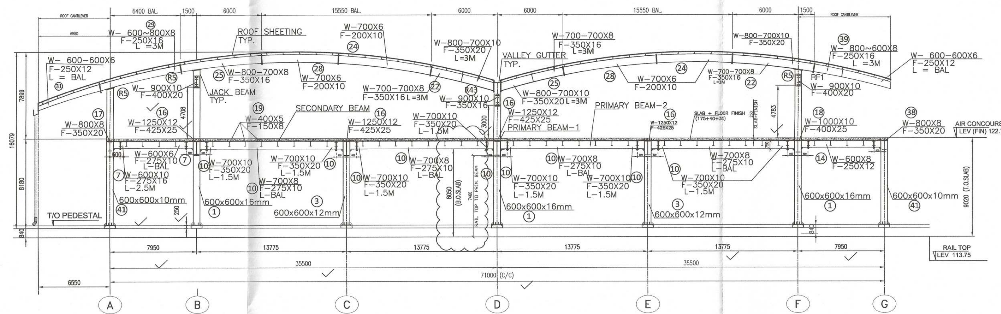
SECTION ALONG GRID-4
