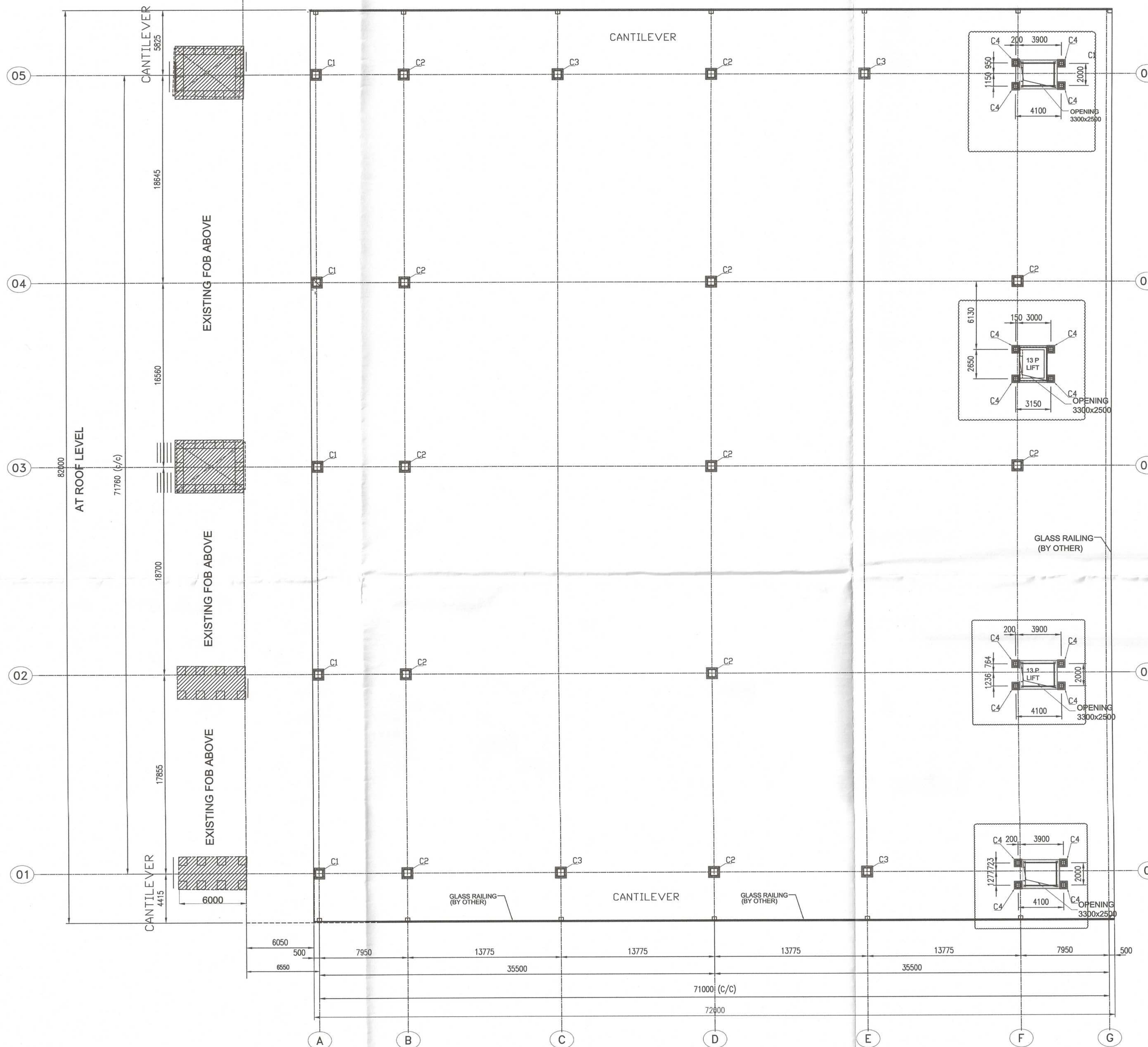
COLUMN LAYOUT PLAN @ CONCOURSE FLOOR LEVEL
