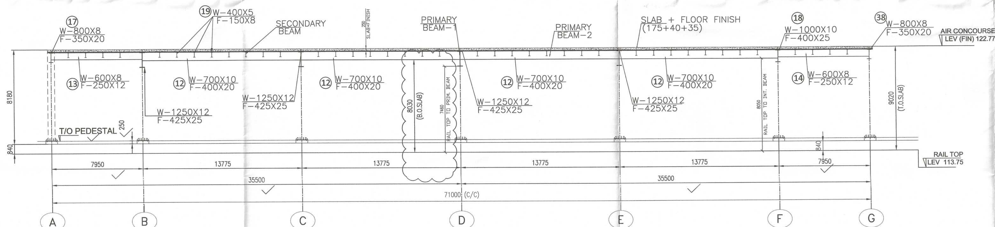
SHOWING PRIMARY BEAM ALONG GRID-PB2 TO PB9
