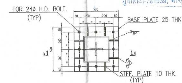
BASE DETAIL FOR STAIRCASE COLUMN MKD. C5
