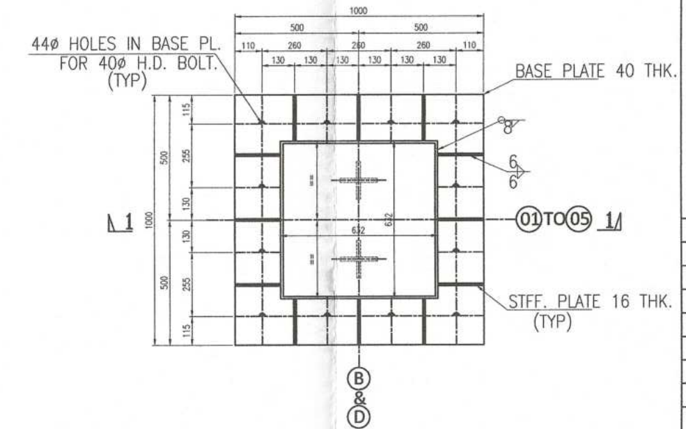
BASE DETAIL FOR COLUMN MKD. C2
