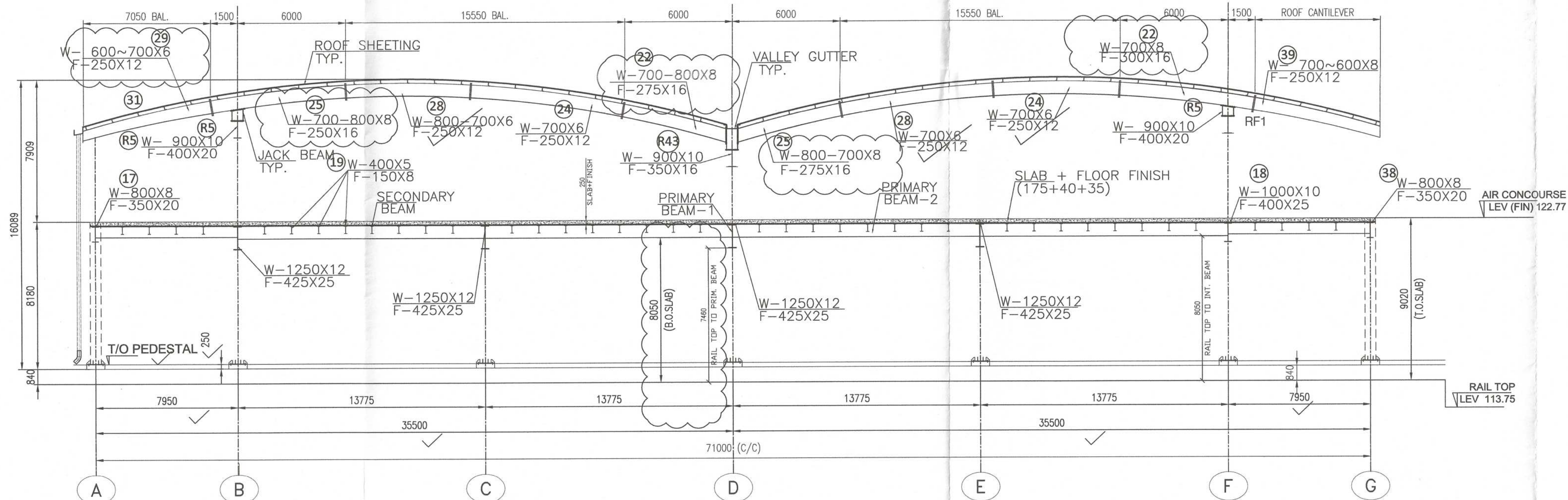
SHOWING JACK BEAM RAFTER ALONG GRID-RF1 RF2 RF3 & RF4
