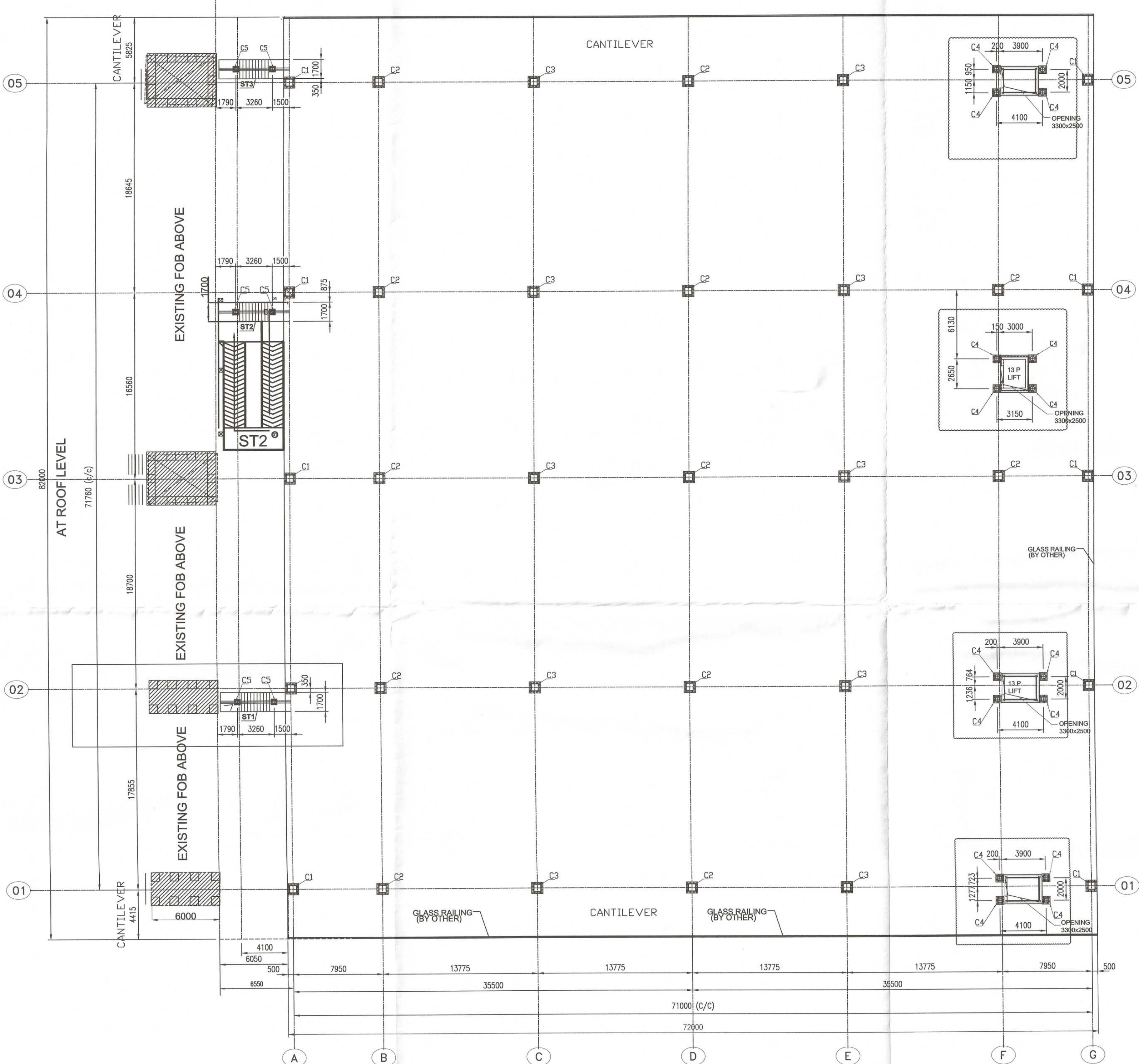
VIEW 2-2
