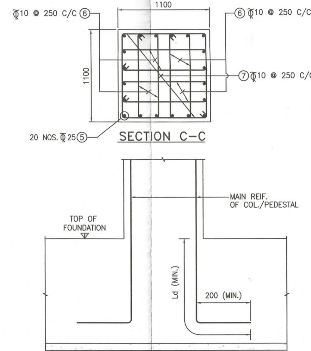
TYPICAL DETAIL OF ANCHORAGE OF COL./PEDESTAL REINFORCEMENT
